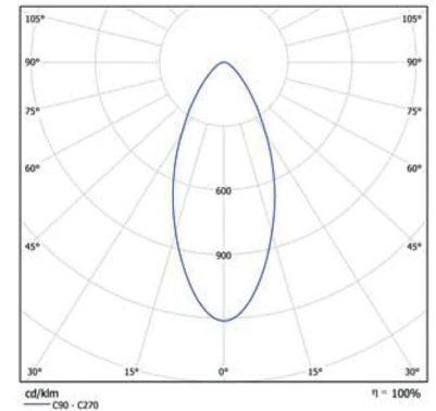
Luminous Intensity Distribution
