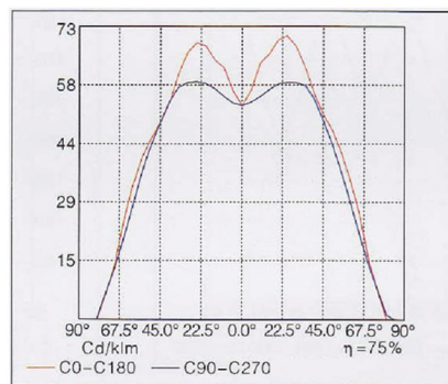
Photometric Curve:
